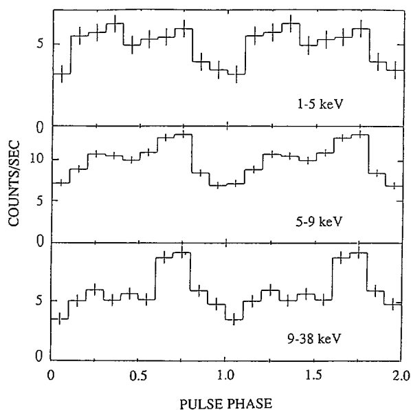
FIG. 1.—Pulse profile of Sct X-1 in three energy bands (1-5, 5-9, and 9-38 keV).
