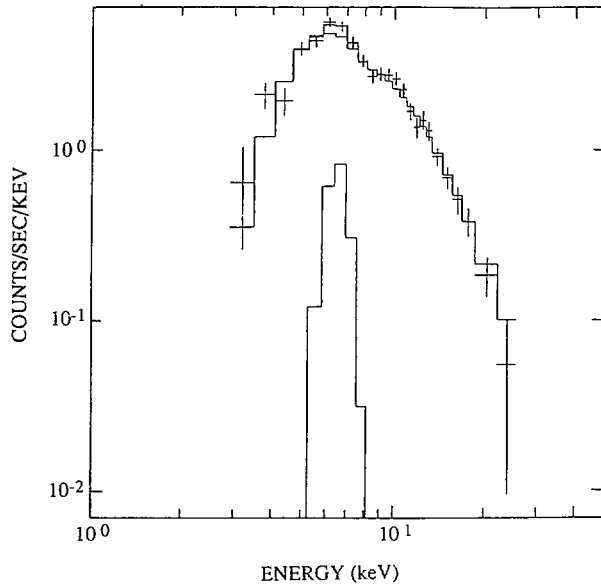
FIG. 3.—Energy spectrum of Sct X-1 from the pointed observation. The solid line represents the best-fit model (see text).
