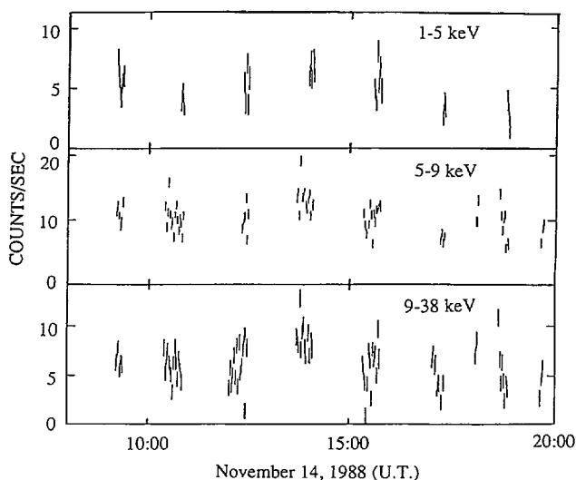
FIG. 2.—X-ray light curve of Sct X-1 in three energy bands (1-5, 5-9, and 9-38 keV). The data in the 1-5 keV band during sunlight portions of the orbit were not included because of a possible contamination from solar X-rays (see text).
