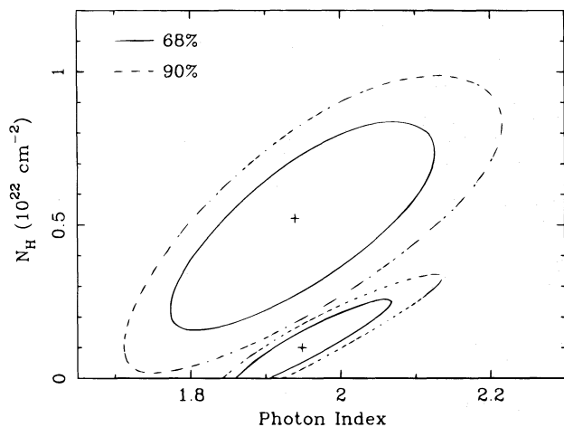
FIG. 4.— \chi^2 contours (90% and 1 \sigma ) for the average 1988 Ginga spectrum and the 1989 Ginga spectrum for a joint fit of the reflection model, allowing the index and absorption to vary. These show that in the context of the reflection model, the spectral variability can be explained by variation in the neutral absorption column.
